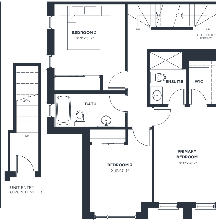
LEVEL 3
